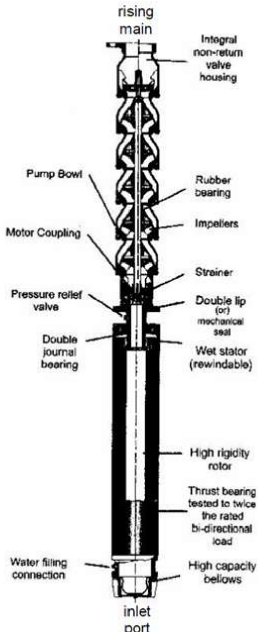
Figure E.10: Submersible Pump (Source: Water Supply Design Manual, 2009)
