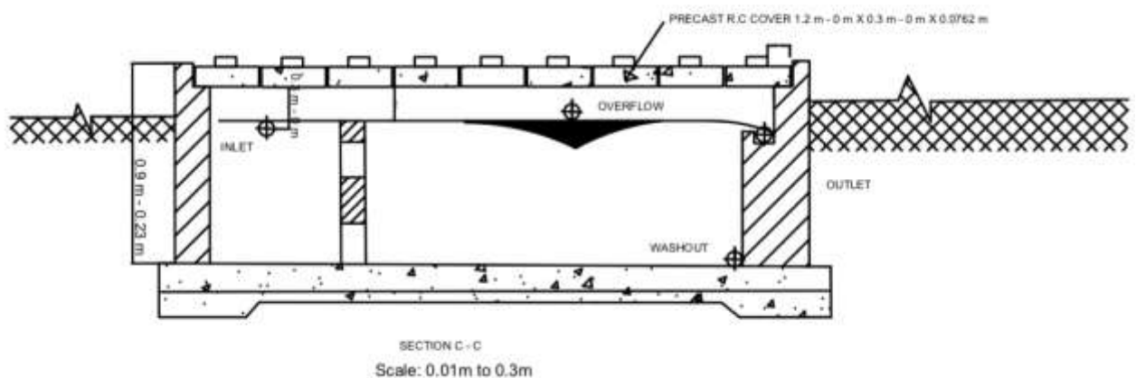
Figure 7.16: Longitudinal cross section
