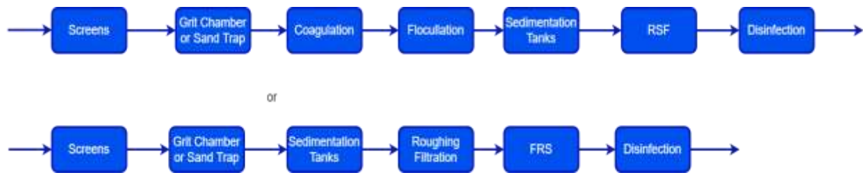
Figure 7.7: Flow sheets for treatment of very turbid surface water or silted lowland stream
