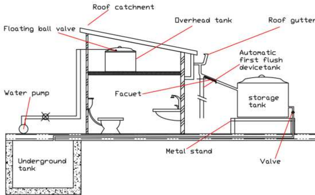
Figure 9.15 Roof Rainwater harvesting system including the storage tank(s)
