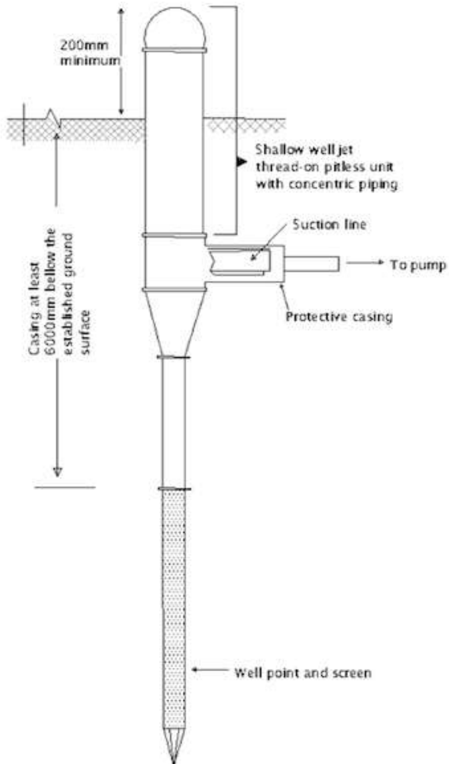
Figure 9.7: Driven wells/IDPH
