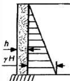
(1) Triangular load (fixed base)
