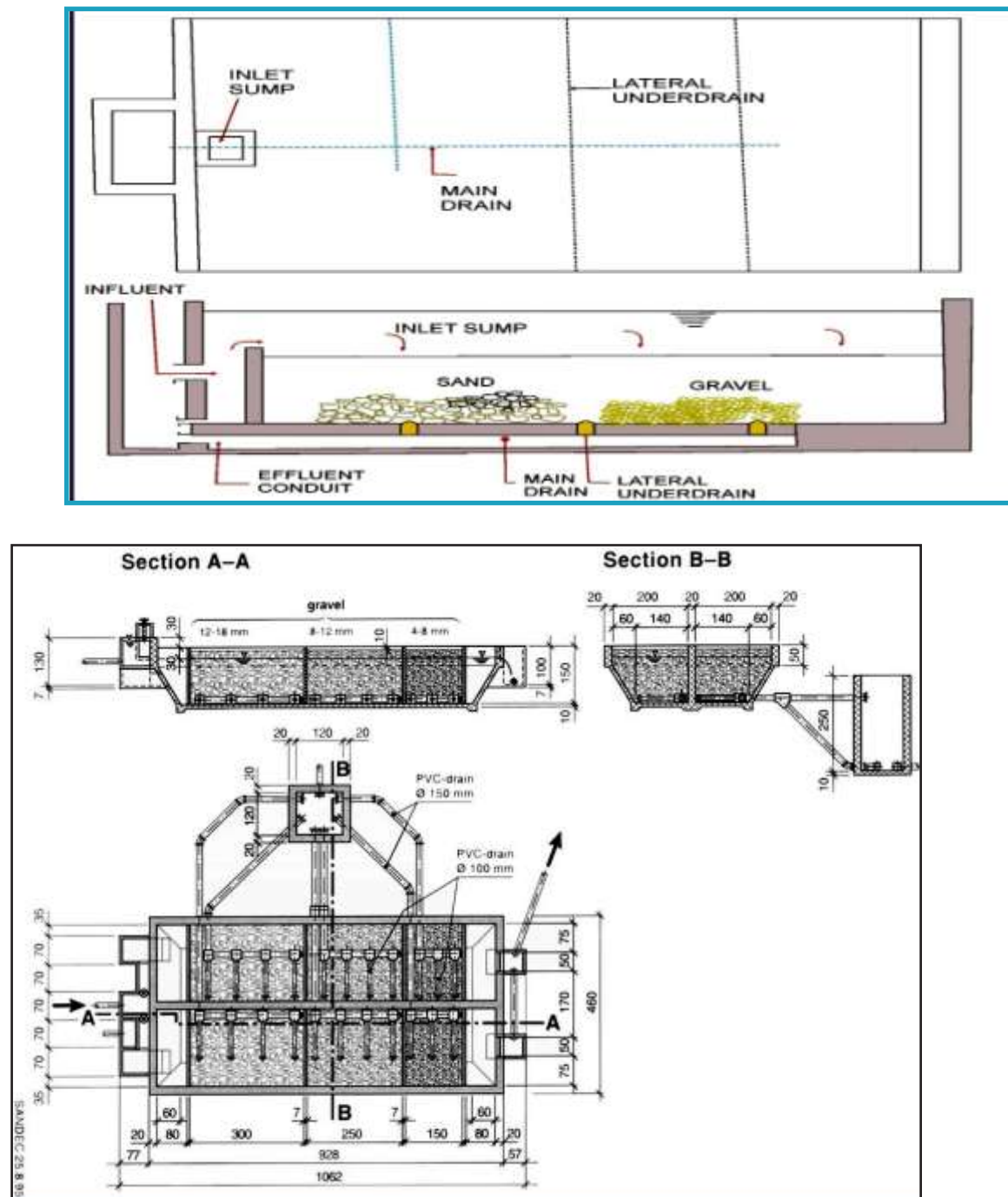
Figure G.1 (a): Layout of Horizontal-Flow Roughing Filter
