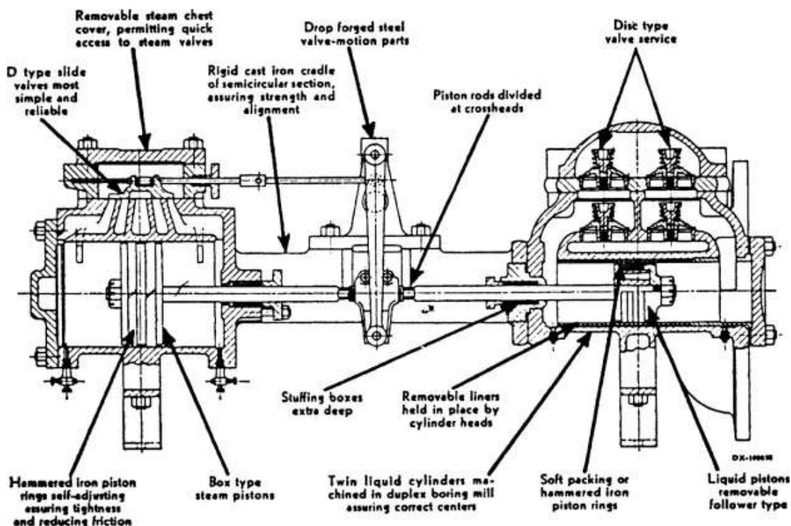
Figure E.6: Duplex – two piston pump 17
