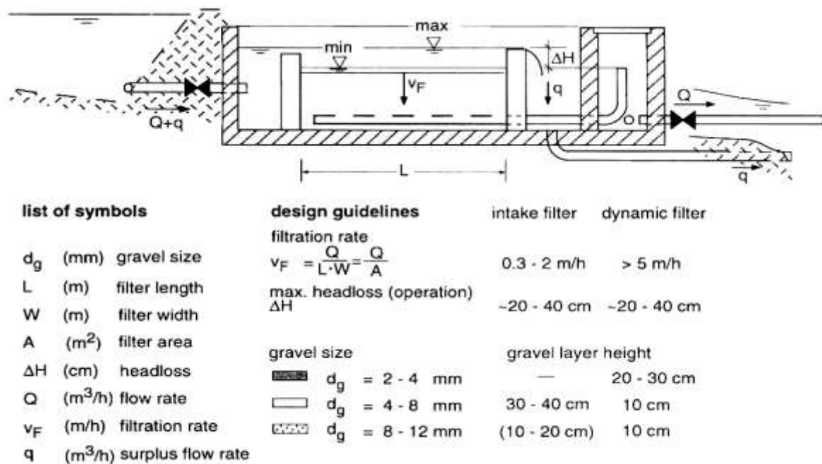
Figure G.3: (c) Layout of the Dynamic intake and Dynamic roughing filter
