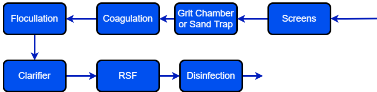
Figure 7.1: Flow sheets for treatment of lake water, dam, reservoir (multiple water intakes)
