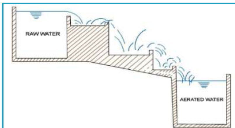
Figure 7.25: Diagram of a Cascade aerator
