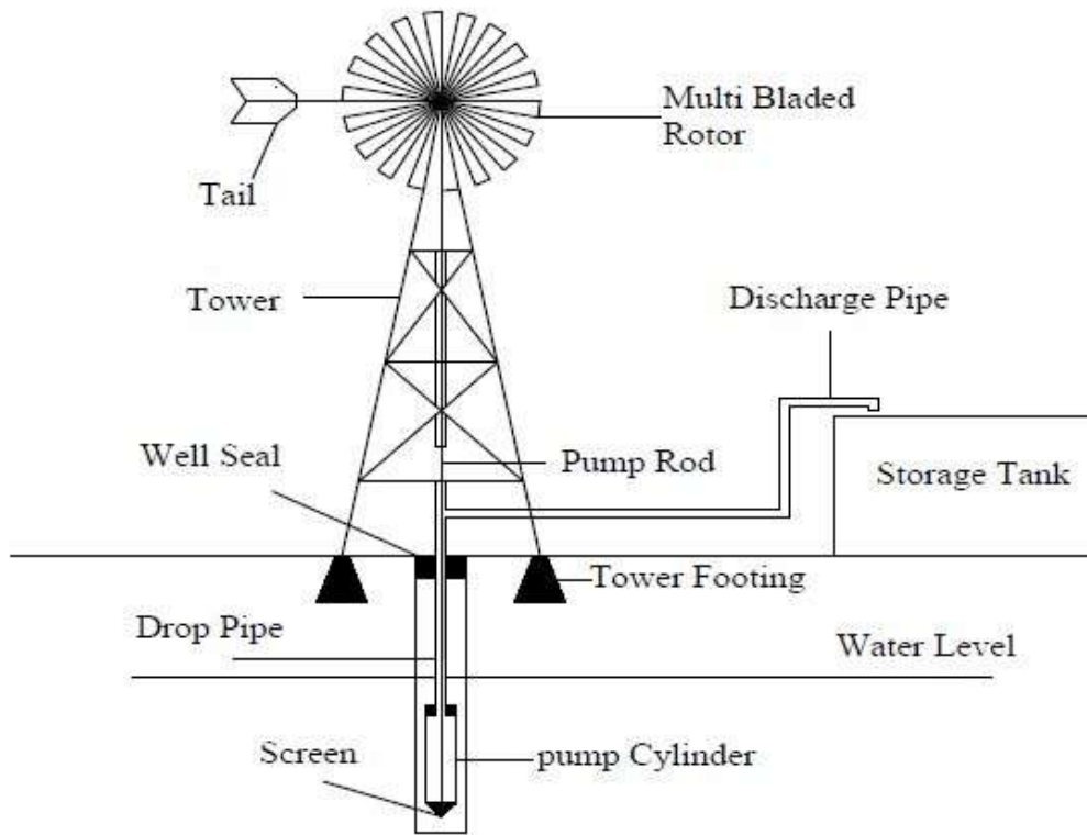
Figure F.3: Windmill driven water pumping 22
