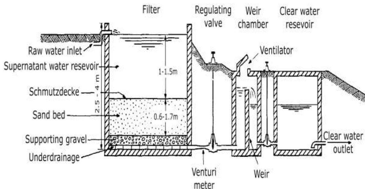
Figure 7.23: (a) A cross section of the Slow Sand Filter (SSF)
