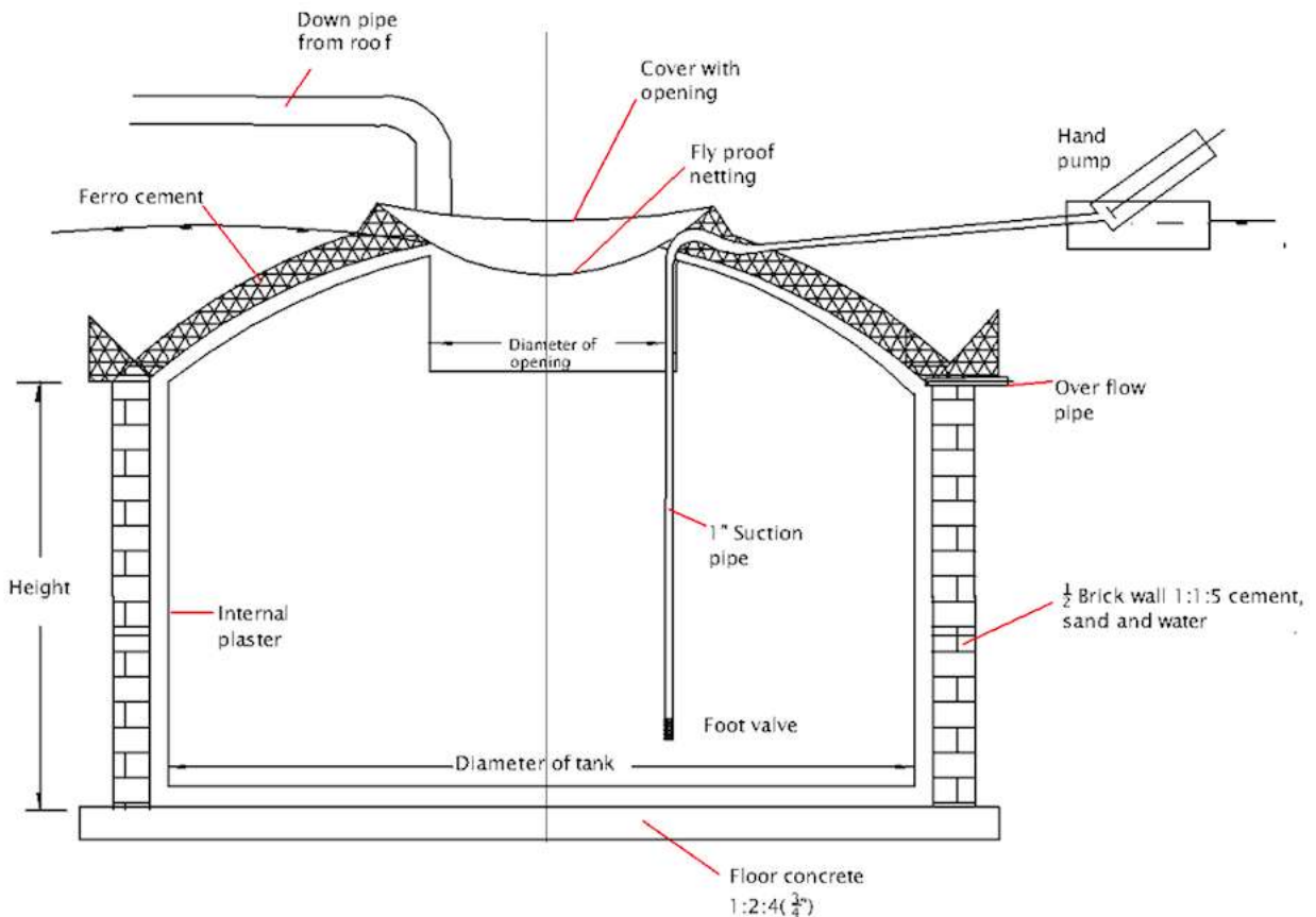
Figure 9.14: Underground Dome shaped Ferro-cement Tank
