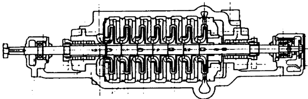
Figure E.3 Axially split multistage pump
