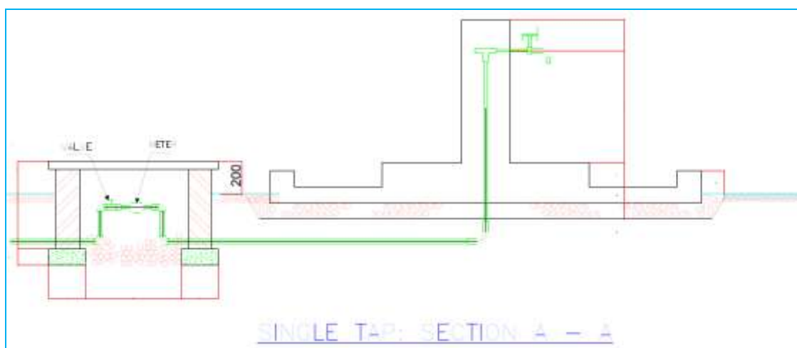
Figure 9.18: Typical Detail of a Single Tap Domestic Point
