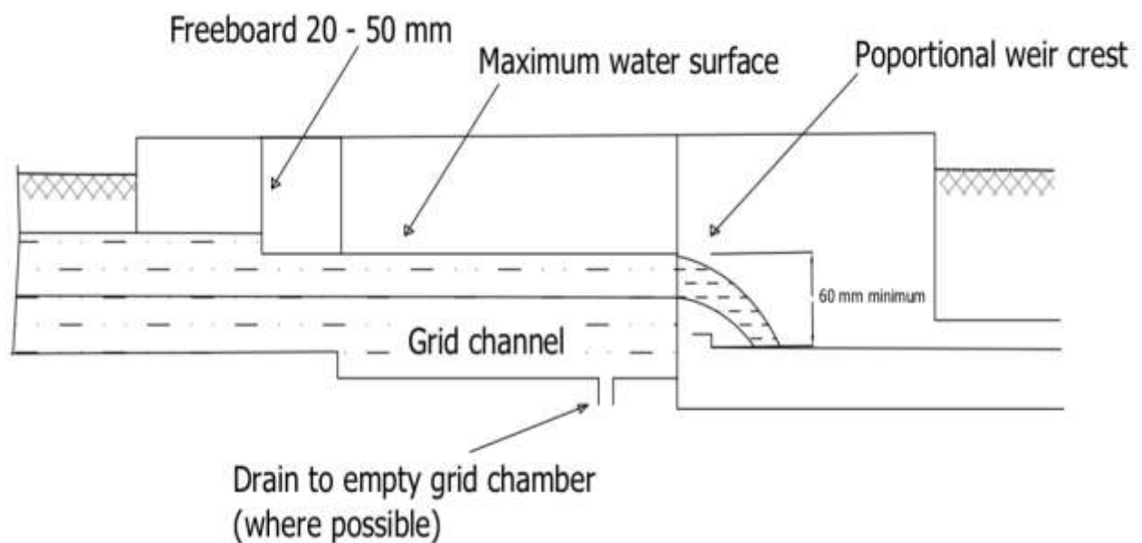
Figure 7.14: Cross Section through the Grit channel
