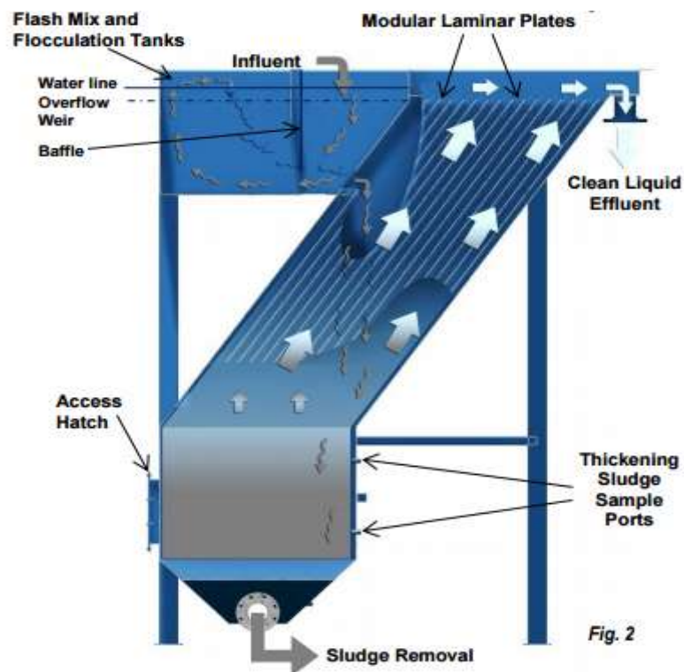
Figure 7.21: Typical Purpose Built Lamella Settle
