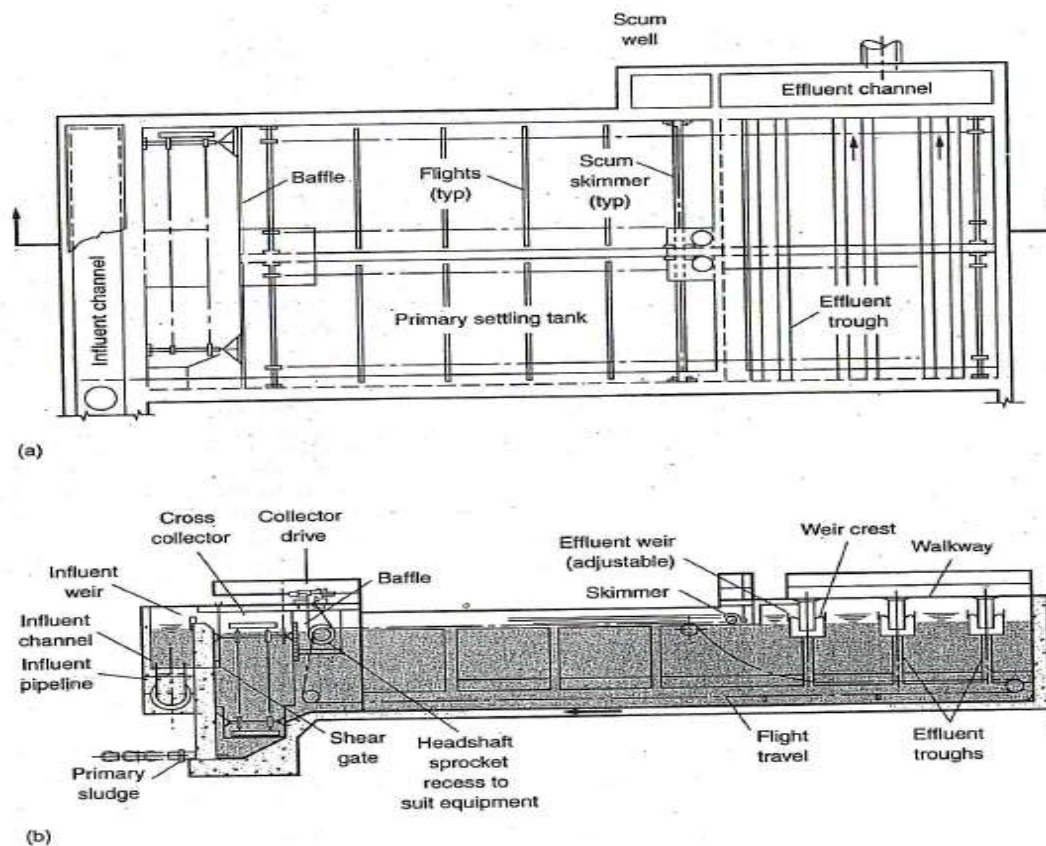
Figure 7.19: Rectangular sedimentation tank
