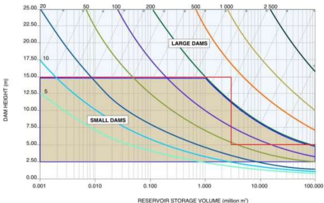
Figure 9.3 Classification of dams according to size
