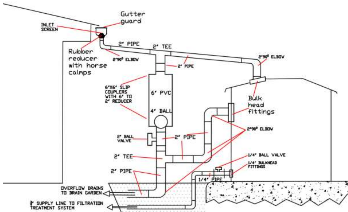
Figure 9.16: Arrangement of the coarse mesh and first flush pipe
