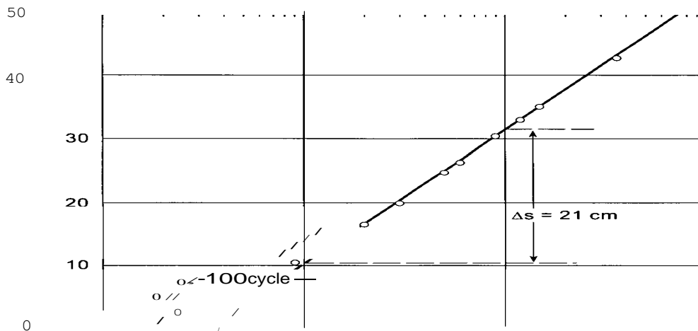
Figure 9.11: A plot of drawdown values s(r,t) against the corresponding time t , on semi-log paper (with t on the logarithmic scale)
