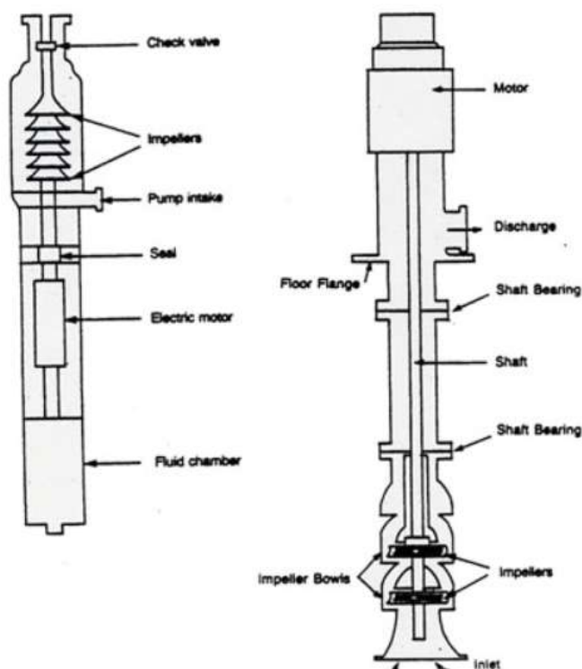
Figure E.9: Turbine pump
