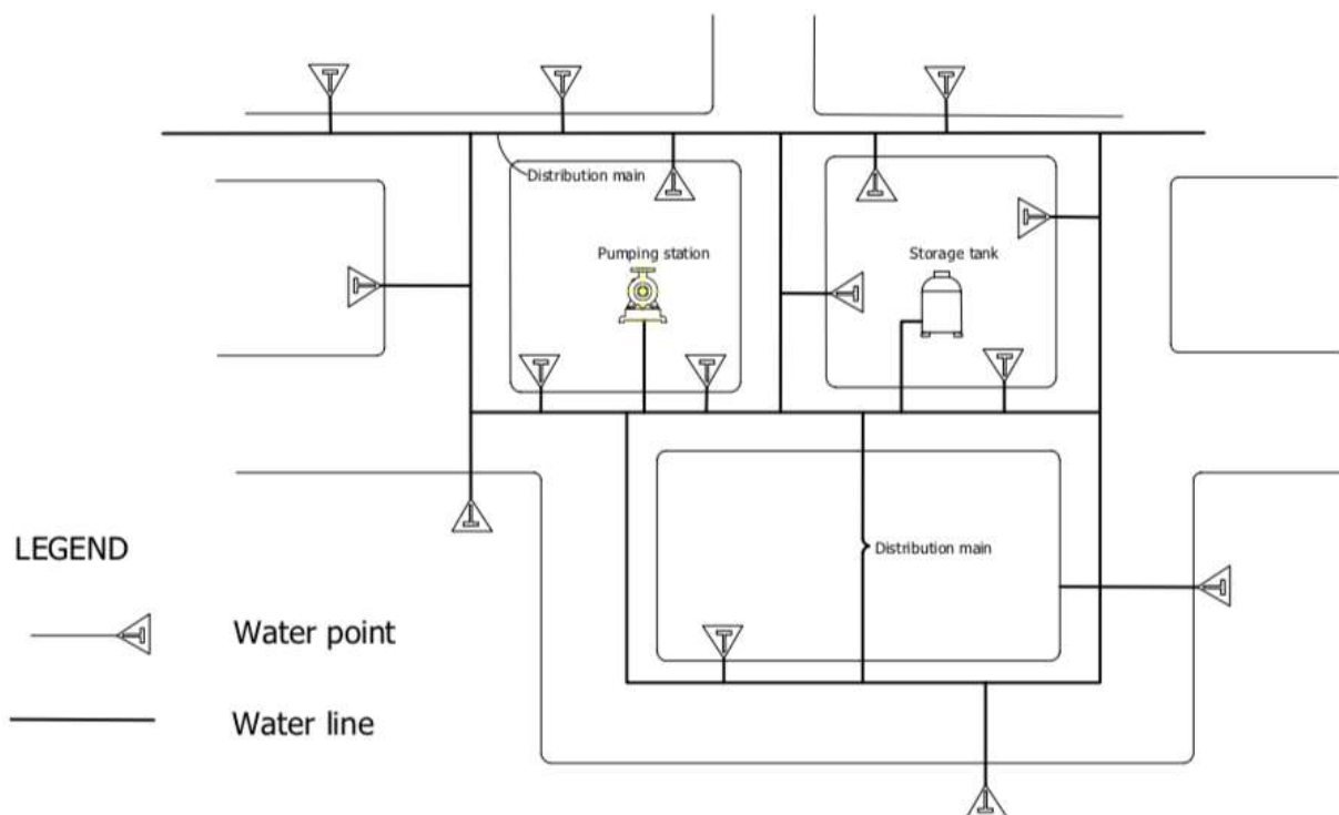
Figure 5.2: Distribution System Basic Layouts
