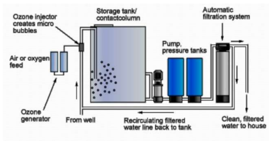
Figure 7.26: Ozonation Process 10
