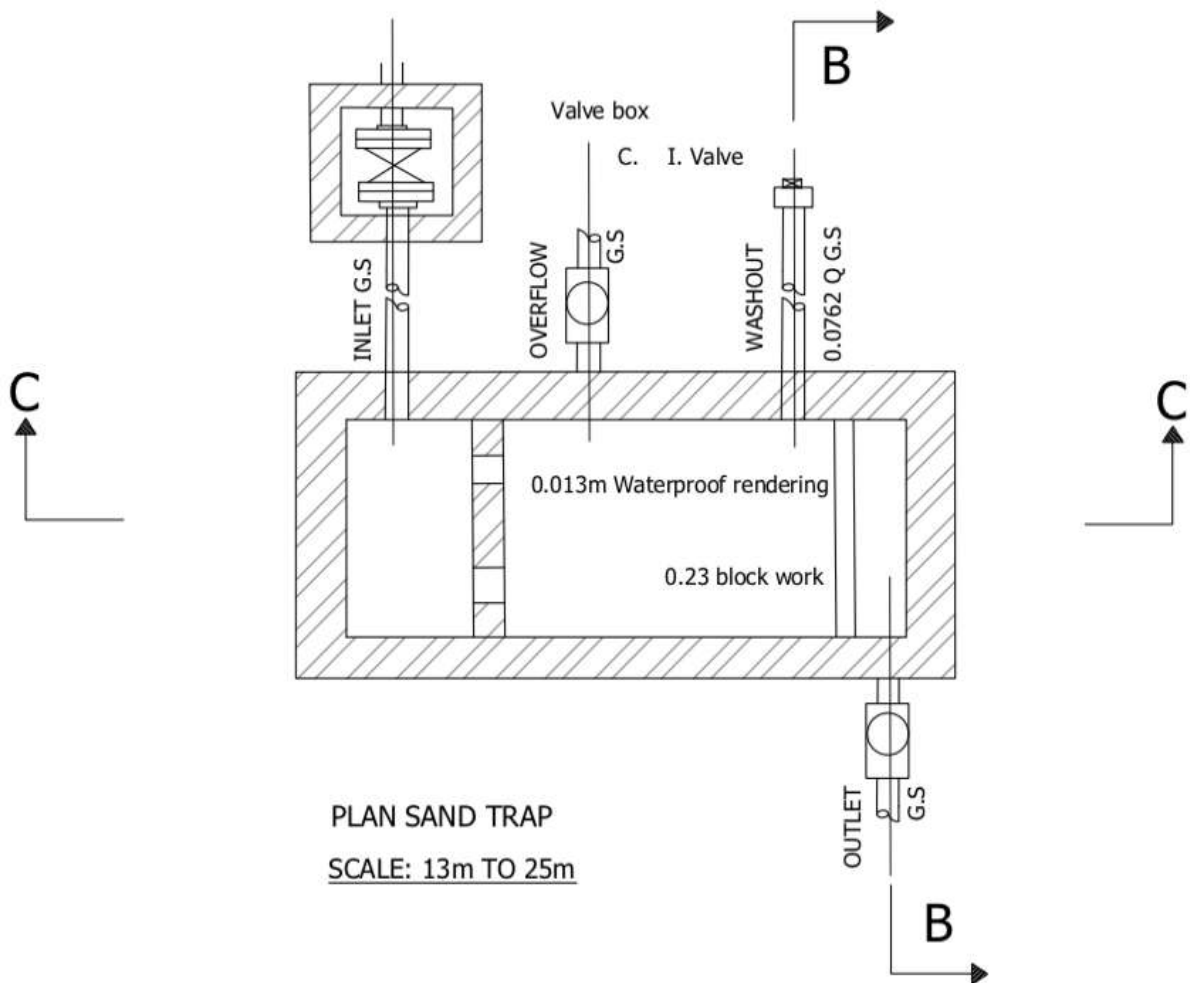
Figure 7.15: Typical layout plan of a sand trap for a small scheme (source: adapted from Philines Rural Water Supply Design Manual , Volumn I, 2012)
