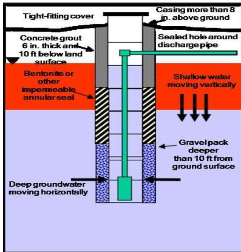
Figure 9.8: A properly bored well construction, not to scale
