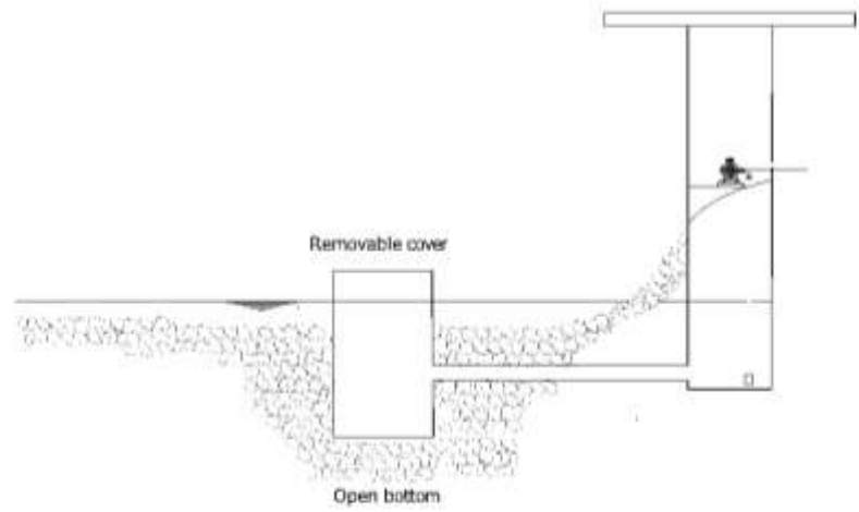
Pumping station in embankment of water abstraction in river bed
