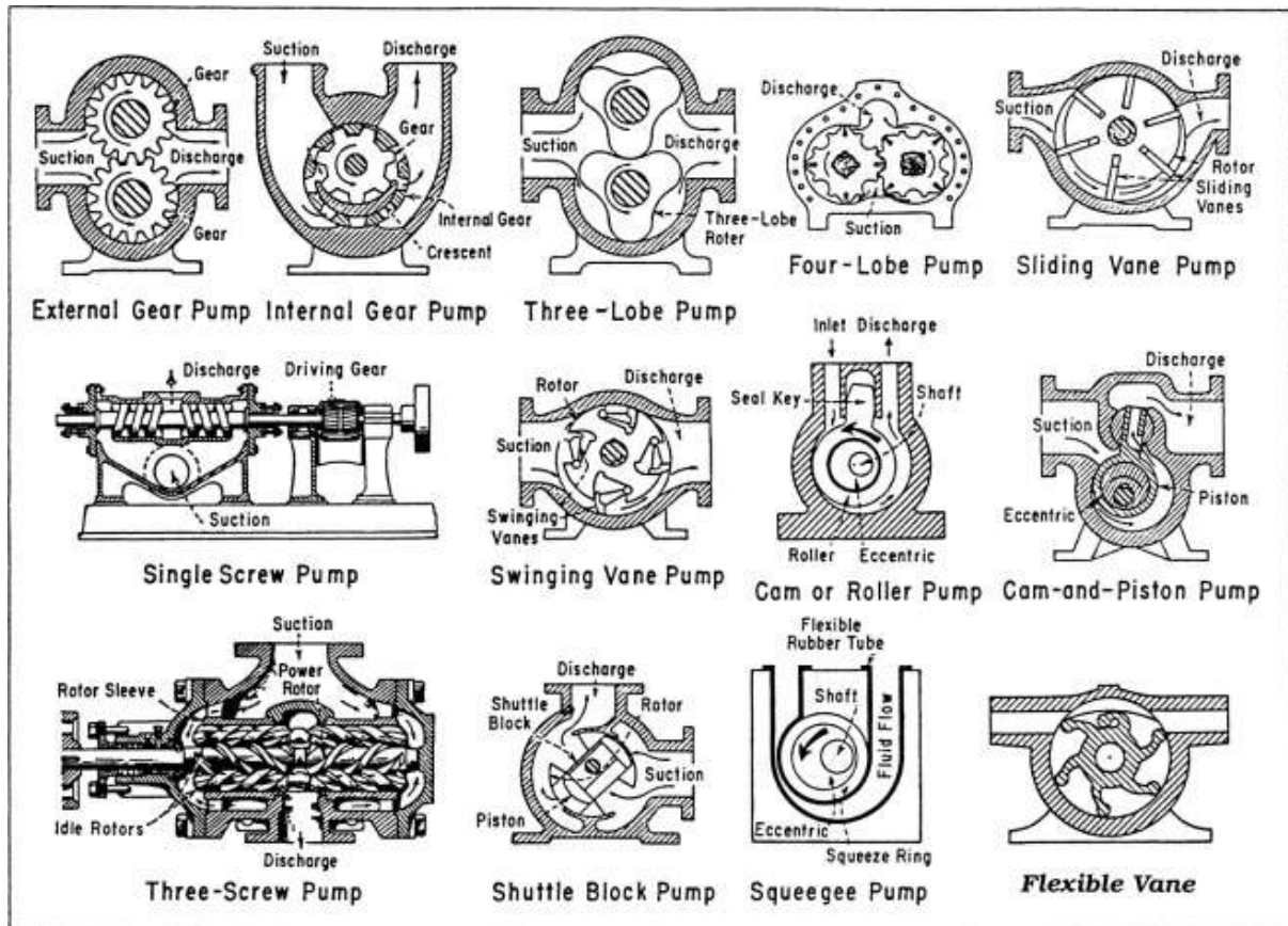
Figure E.8: Types of Rotary Pumps(Coker, 2014 #2381)
