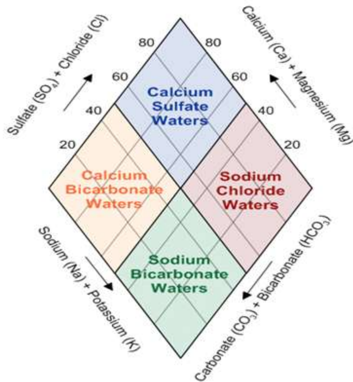
Figure 9.13: Interpretation of the diamond plot
