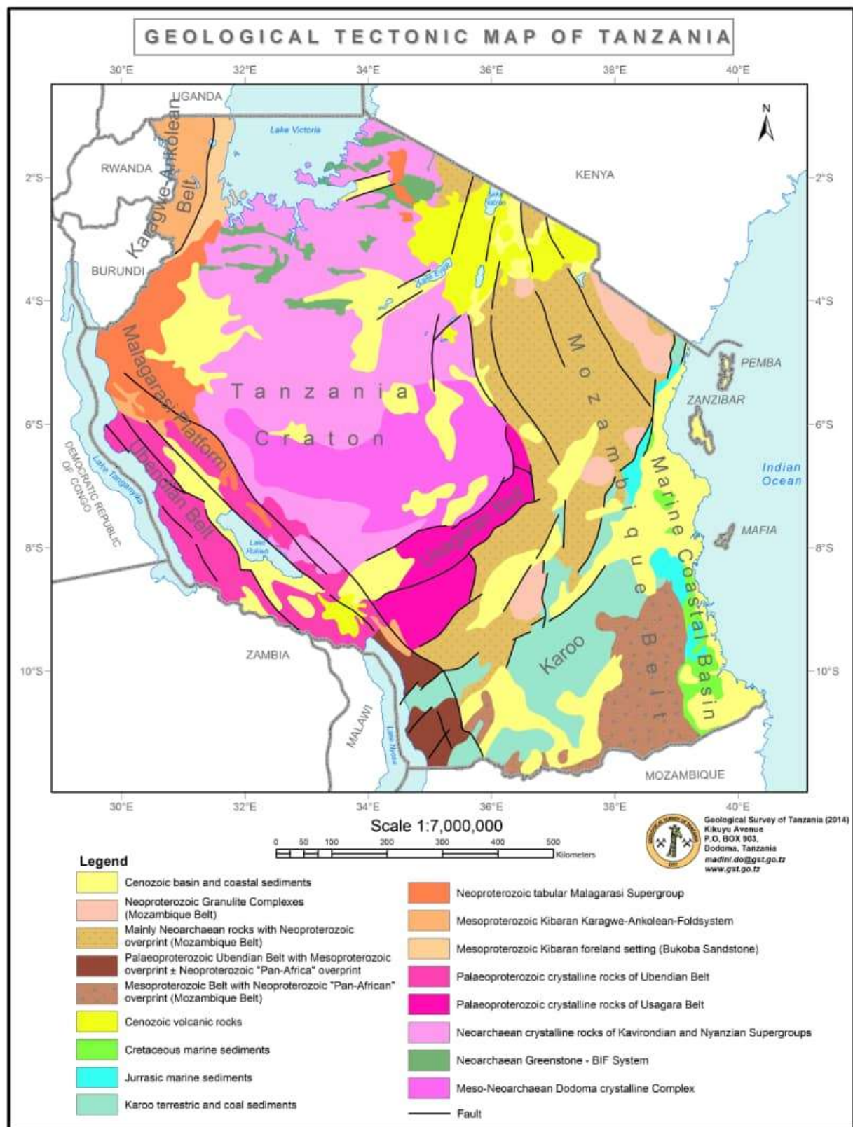
Figure 9.5: Geological Map of Tanzania
