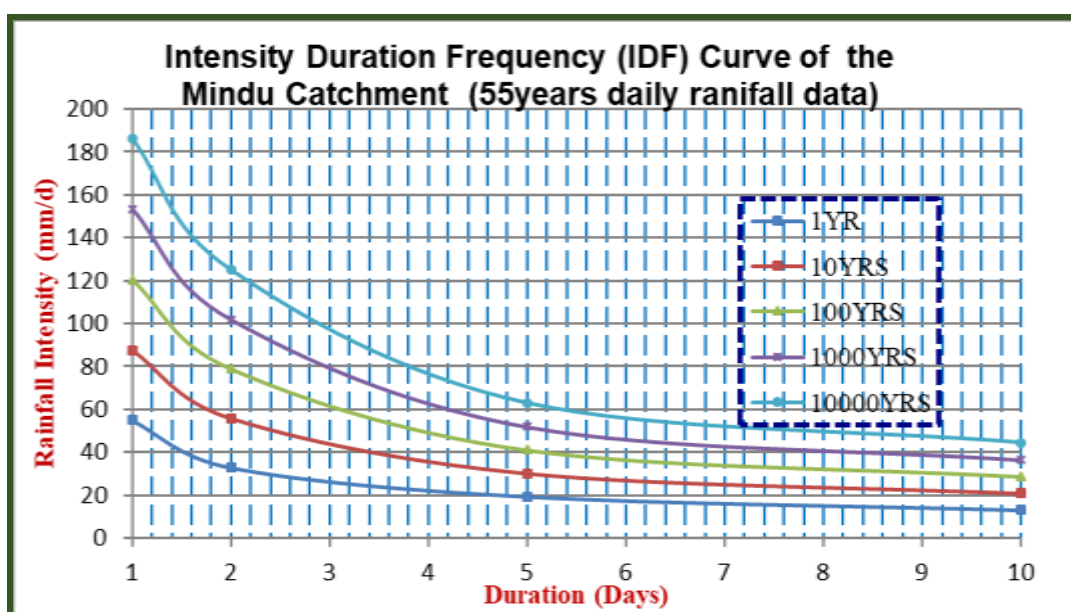
Figure J.2 Typical Example IDF Curve
