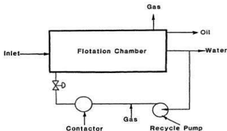
Figure 7.24: A diagram of Dissolved –air flotation mechanism
