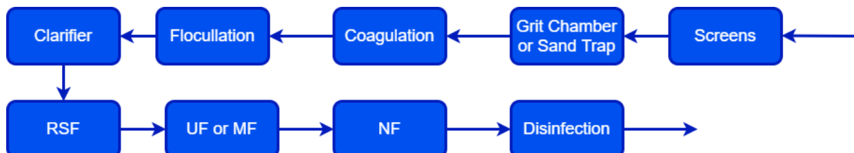
Figure 7.5: Flow sheers for treatment of upland stream with no soil erosion
