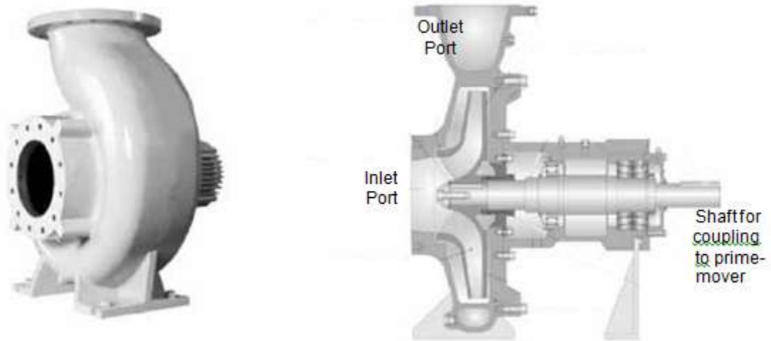
Figure E.2: Section through single stage end suction centrifugal pump
