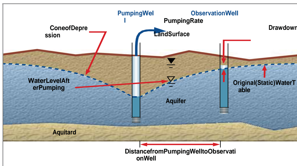
Figure 9.10: Impact of a pumping well on the water table and observation well in an unconfined aquifer
