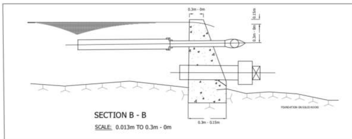
Figure 7.17: Transverse cross section
