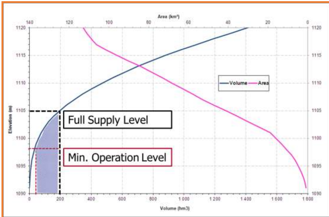
Figure 9.4: Typical A-V-H curve of the reservoir
