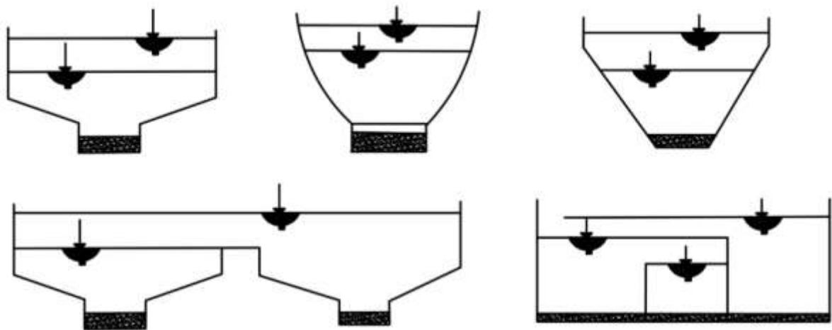
Figure 7.12: Single and Common Section Type of Grit Channels (Source: Poppel, 1982)
