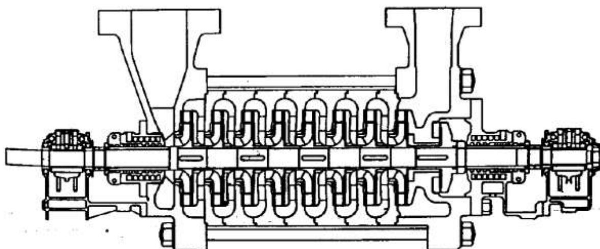
Figure E.4: Radially split ring section multistage pump
