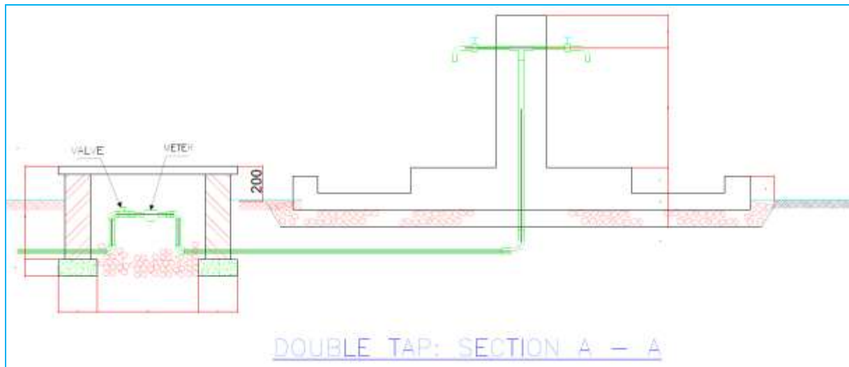
Figure 9.19: Typical Detail of a Double Tap Domestic Point
