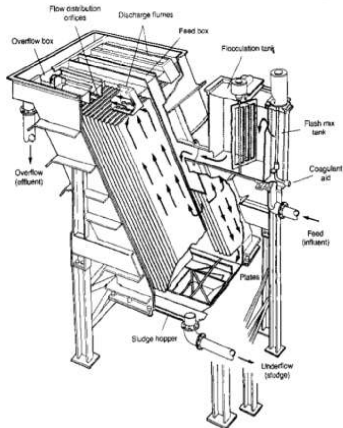
Figure 7.20: Typical Purpose Built Lamella Settler
