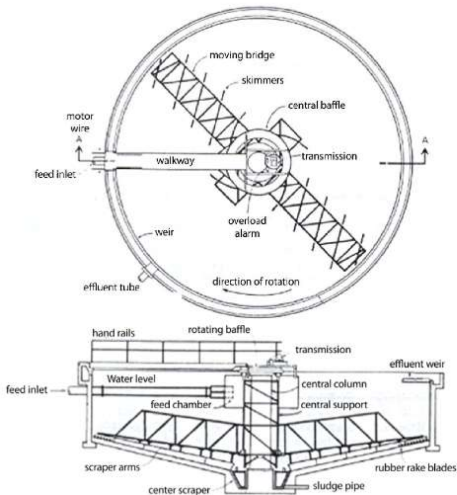
Figure 7.27: Gravity thickener plan and height
