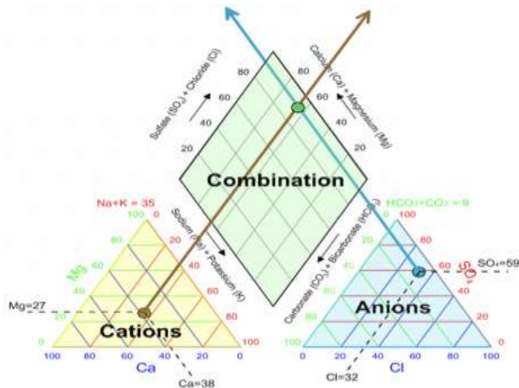
Figure 9.12: The three components of the piper plot
