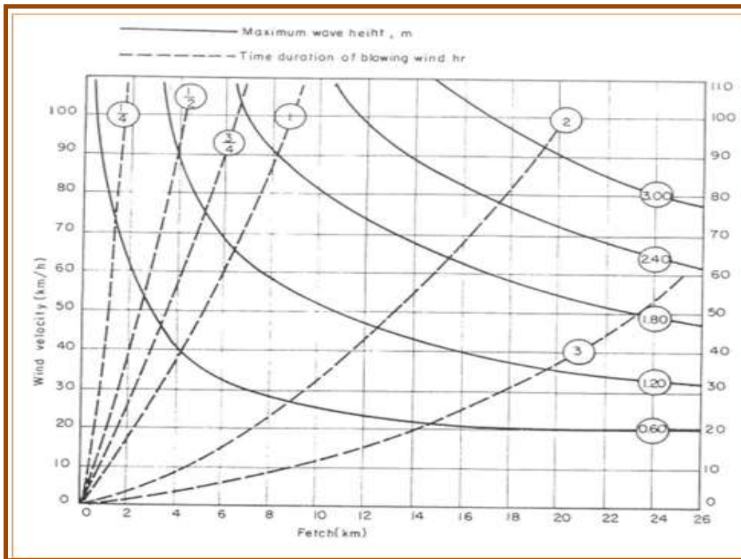
Figure K.1: USACE curve for interpolation of wave height
