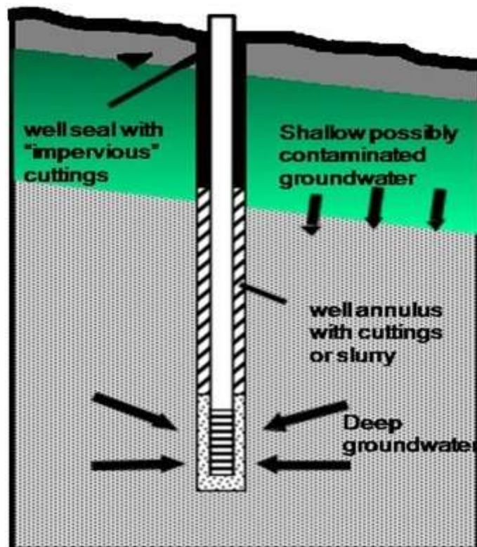
Figure 9.9: Deep Drilled well construction
