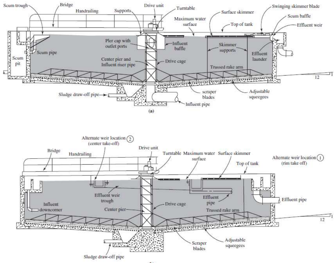
Figure 7.18: Cylindrical sedimentation tank
