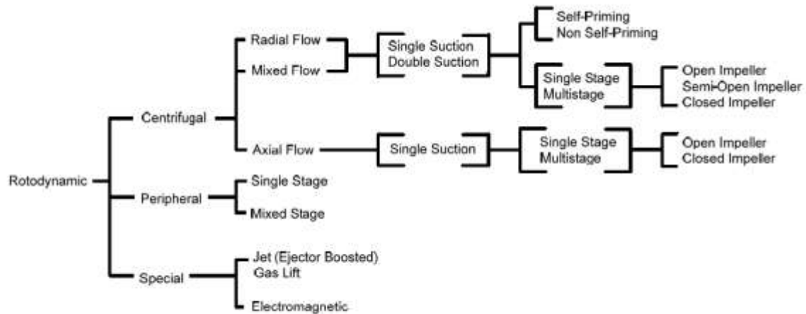
Figure E.1: Classification of Rotary pumps (Source: MoW Design Manual, 2009, 3 rd Edition).
