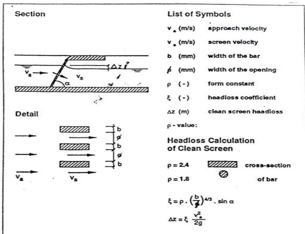
Figure7.10: The Head loss Calculation Formula Through Screens (Source: Poppel, 1982).
